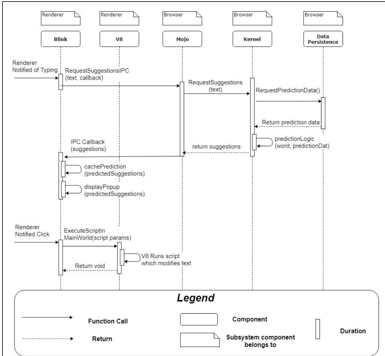
Figure 3: Sequence diagram of requesting, caching, and displaying suggested words, followed by a sequence in which the user has clicked a suggestion, and our feature modifies the typed text.
